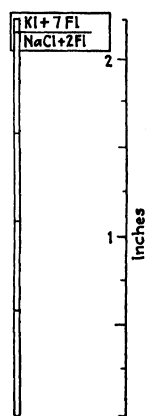
FIG. 3.— Diagram of filled specimen tube.
